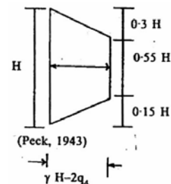
3. (Peck, 1943)
